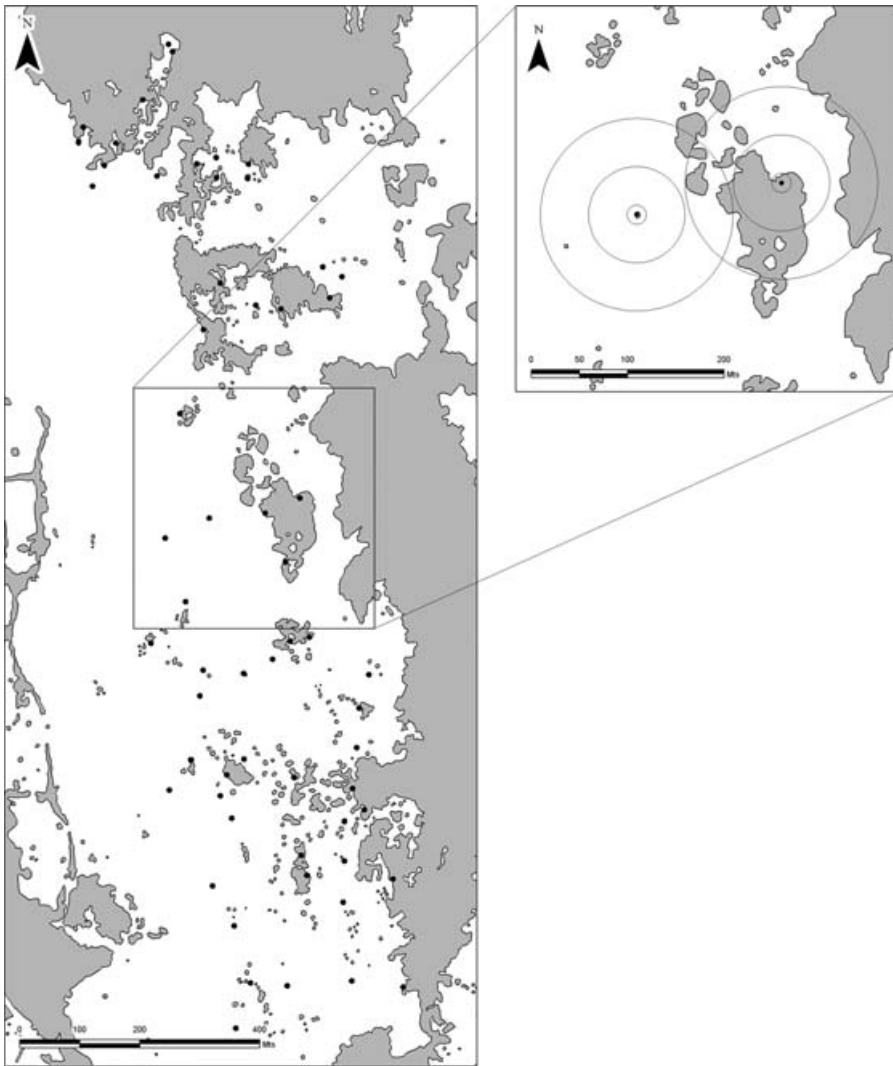
Figure 1. Position of sampled focal trees (black dots) and the configuration of forest cover (grey patches). The enlarged area shows the concentric circles of 10-, 50-, and 100-m radii used to establish the tree-cover sampling plots at different spatial scales.
