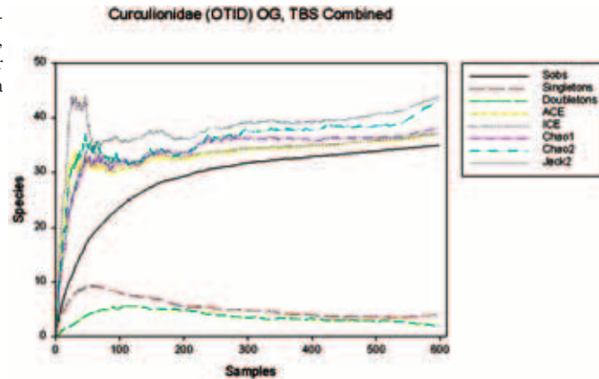
FIGURE 2. Observed species accumulation curve and five estimation curves (ACE, ICE, CHAO 1, CHAO 2, JACK 2) for Curculionidae (Otid) with data combined from both sites.
